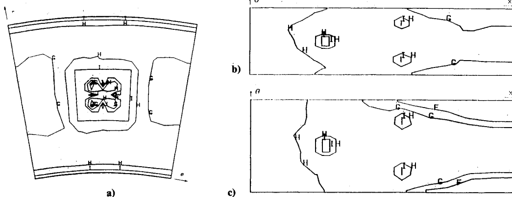
Fig. 5 Wall temperature distribution ( p = 15 bar): a) combustor backplate; b) inner annulus wall; and c) outer annulus wall [contour levels (K): F = 1100; G = 1000; H = 800; I = 600; and J = 500].
