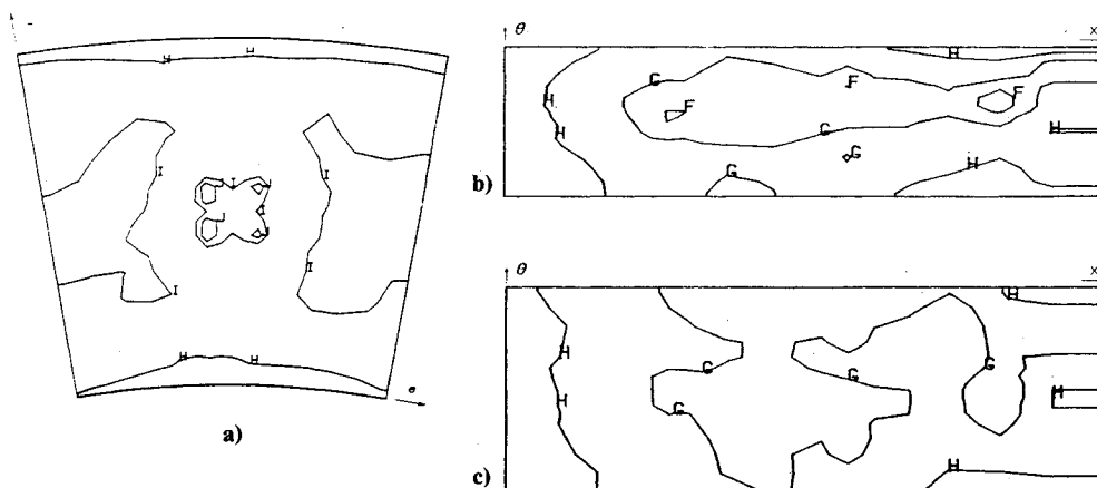
Fig. 3 Radiative wall heat fluxes ( p = 5 bar): a) combustor backplate; b) inner annulus wall; and c) outer annulus wall [contour levels ( \text{kW/m}^2 ): F = 150.0; G = 100.0; H = 50.0; I = 25.0; and J = 10.0].
