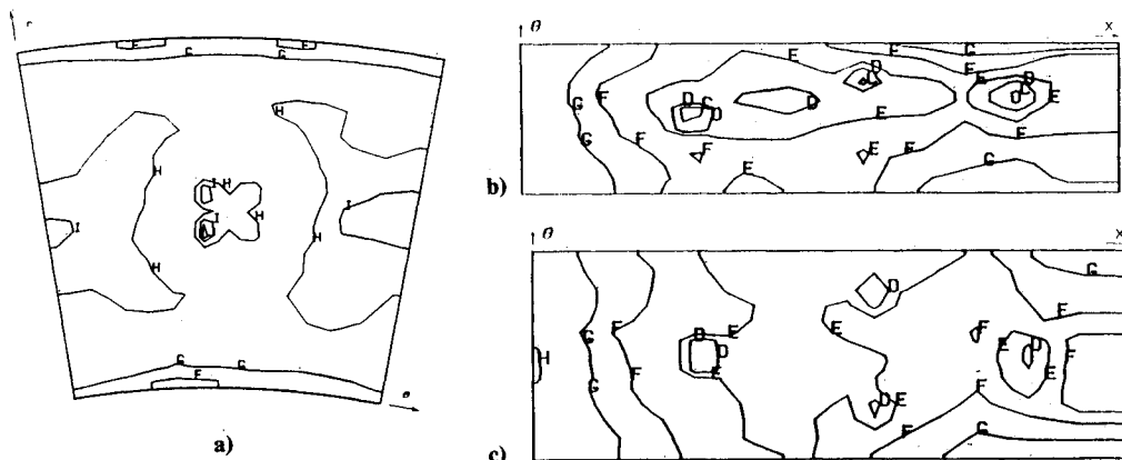
Fig. 6 Radiative wall heat fluxes ( p = 15 bar): a) combustor backplate; b) inner annulus wall; and c) outer annulus wall [contour levels ( \text{kW/m}^2 ): C = 300.0; D = 250.0; E = 200.0; F = 150.0; G = 100.0; H = 50.0; I = 25.0; and J = 10.0].
